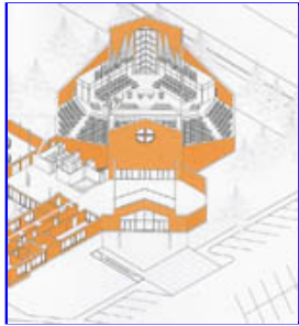
Axonometric of sanctuary
